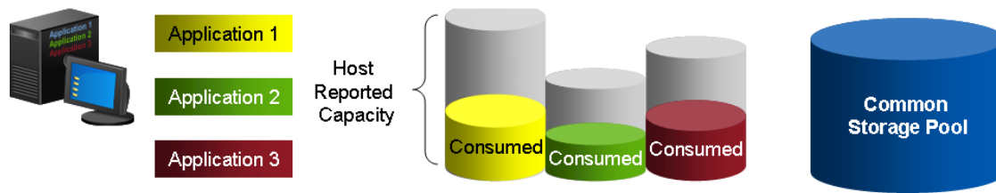
Figure 3. Virtual Provisioning
