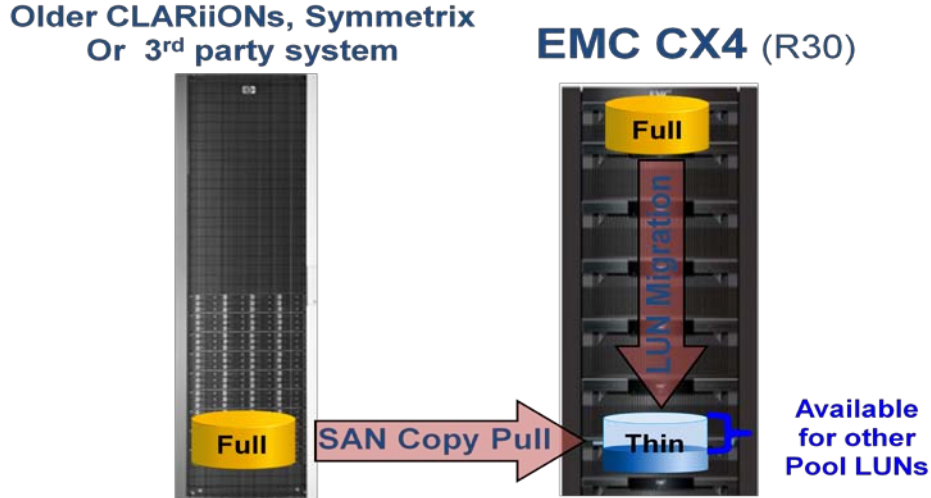
Figure 10. Space reclamation
